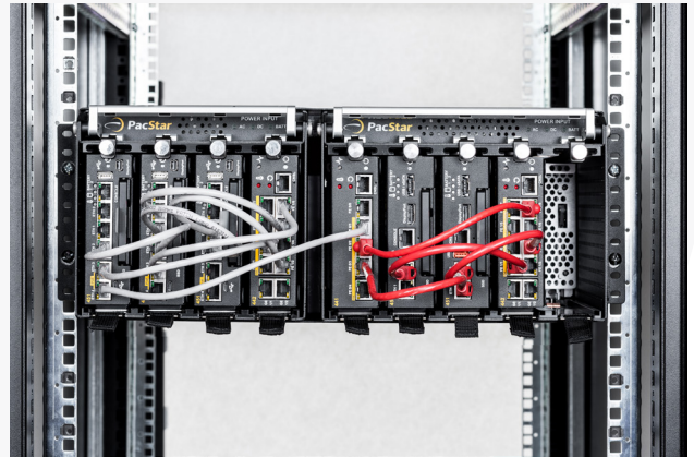
PacStar Modules in 19" Rack, with Rack Mount Frame and 4- and 5-slot PacStar Smart Chassis
