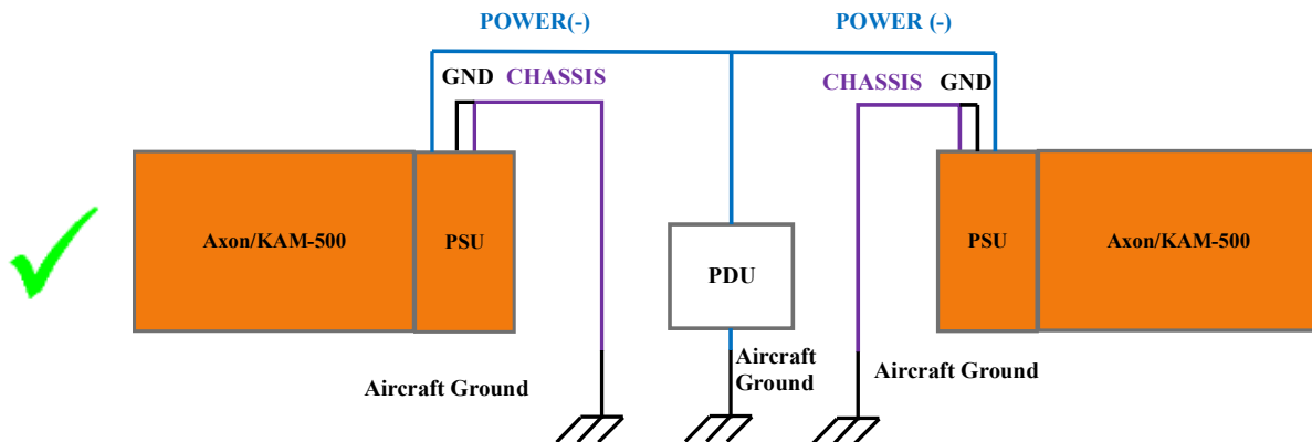
Figure 36-10: How to ground two chassis: Ideally each chassis should have its own connection to the star point
