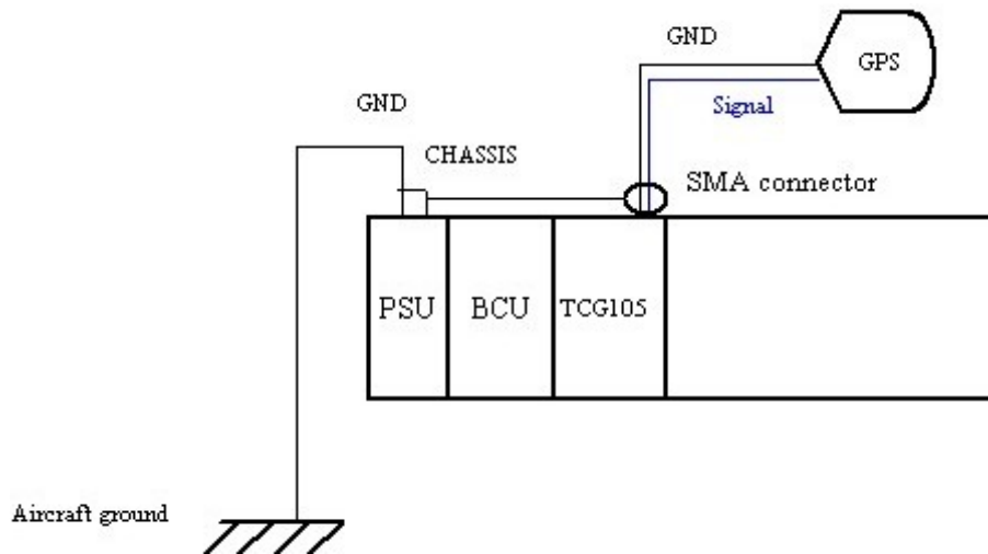
Figure 36-12: KAM-500 grounding with KAD/TCG/10x module and GPS antenna
