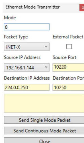
Figure 54-6: Example showing how to erase a KAM/MEM/113 by setting format 8 using the Ethernet Mode Transmitter tool
