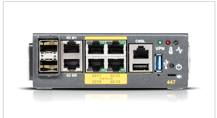
Figure 1: PacStar 447 Small Router Module with Cisco ESR 6300
