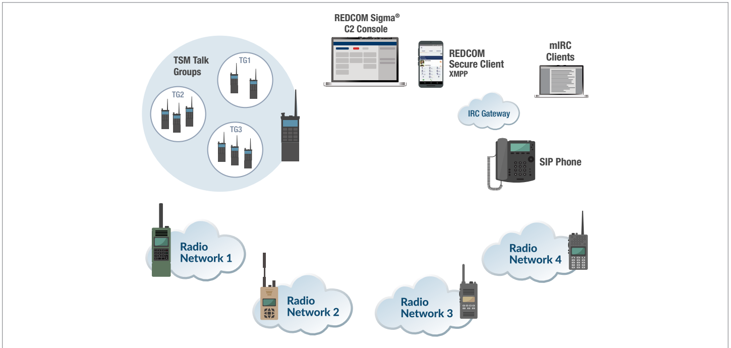
Figure 1: Product block diagram
